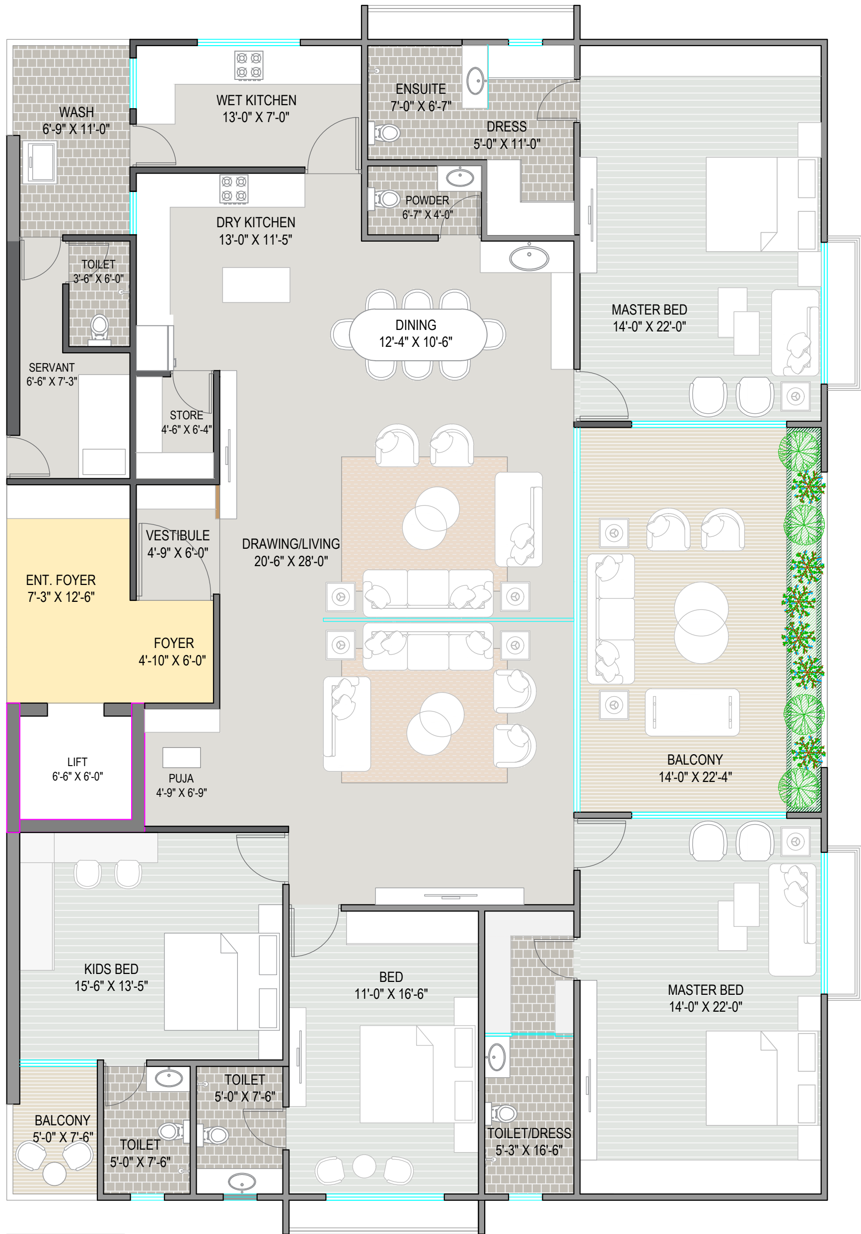
TYPICAL FLOOR PLAN UNIT B AREA - 283.55 SQ.MTS.
